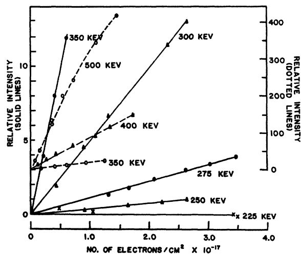
FIG. 2. Intensity of the fluorescence in wavelength region 5400–5500 Å as a function of bombardment and electron energy.
